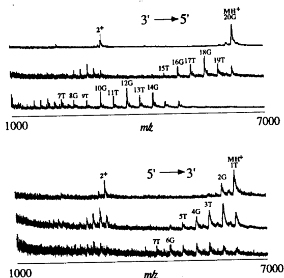
Figure 1. Positive ion MALDI-MS of a ladder sequence from a 20 mer oligonucleotide from the 3' to 5' end with SVP (top) and 5' to 3' end with BSP (bottom). The order of the peaks corresponds to the sequence. Snake venom phosphodiesterase (SVP) digests the DNA from 3' to 5'. Bovine spleen phosphodiesterase (BSP) digests the DNA from 5' to 3'.
