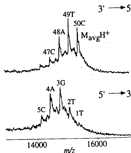
Figure 2. Positive ion MALDI-MS ladder sequence from a digest of a 50 residue oligonucleotide. It was sequenced from the 3' to 5' and from the 5' to 3'.
