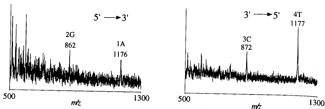
Figure 5. Positive ion MALDI-MS data generated from the oligonucleotide 5'-AGCT-3' using the ladder sequencing approach. T BSP digest is shown on the left, while the SVP digest is shown on the right.
