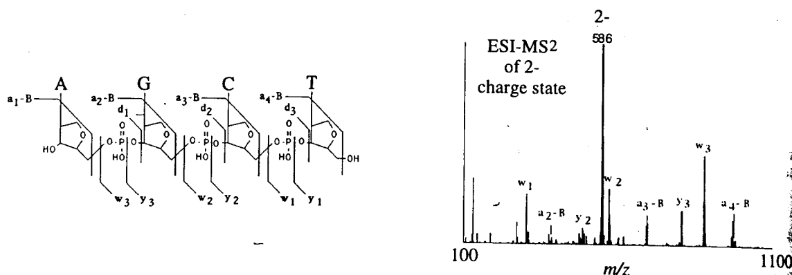
Figure 6. Negative ion electrospray ionization-MS 2 data generated in the oligonucleotide 5'-AGCT-3'. Cleavage of base, sugar, and phosphate were all observed in these experiments.
