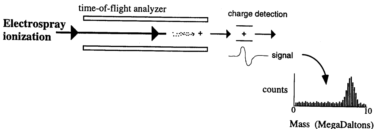
Figure 10. A time-of-flight mass analyzer with charge (inductive) detection was used by Fuerstenau and Benner 28 and Park and Callahan 39 to perform charge detection mass spectrometry. Fuerstenau and Benner used an electrospray ionization source on their instrument to mass measure megadalton DNA and, more recently, to measure whole viruses (unpublished data).
