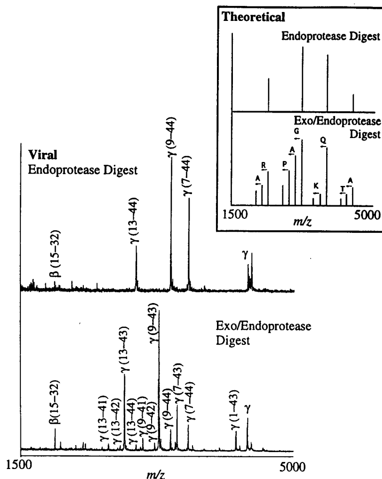
Figure 4. Digestion of Flock House viral capsid proteins, performed directly on the virus. (Top) MALDI/MS data generated from the trypsin digest. (Bottom) data generated from the carboxypeptidase Y digest of the trypsin digest (or endo/exo sequential digestion) of the viral capsid protein. The numbers in parentheses corresponds to viral protein fragments. (Inset) theoretical exoprotease digestion and a theoretical exo/endo -protease digestion; 1 the single-letter code correspond to amino acids in the peptide sequence.
